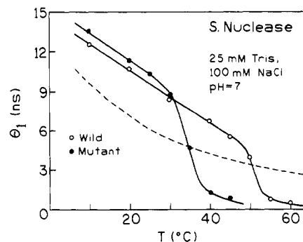
FIGURE 9: Temperature dependence of the overall ( \Theta_1 ) correlation times for wild-type nuclease (O) and mutant nuclease-conA-SG28 (●). The dashed line shows the temperature dependence of \eta/T .
